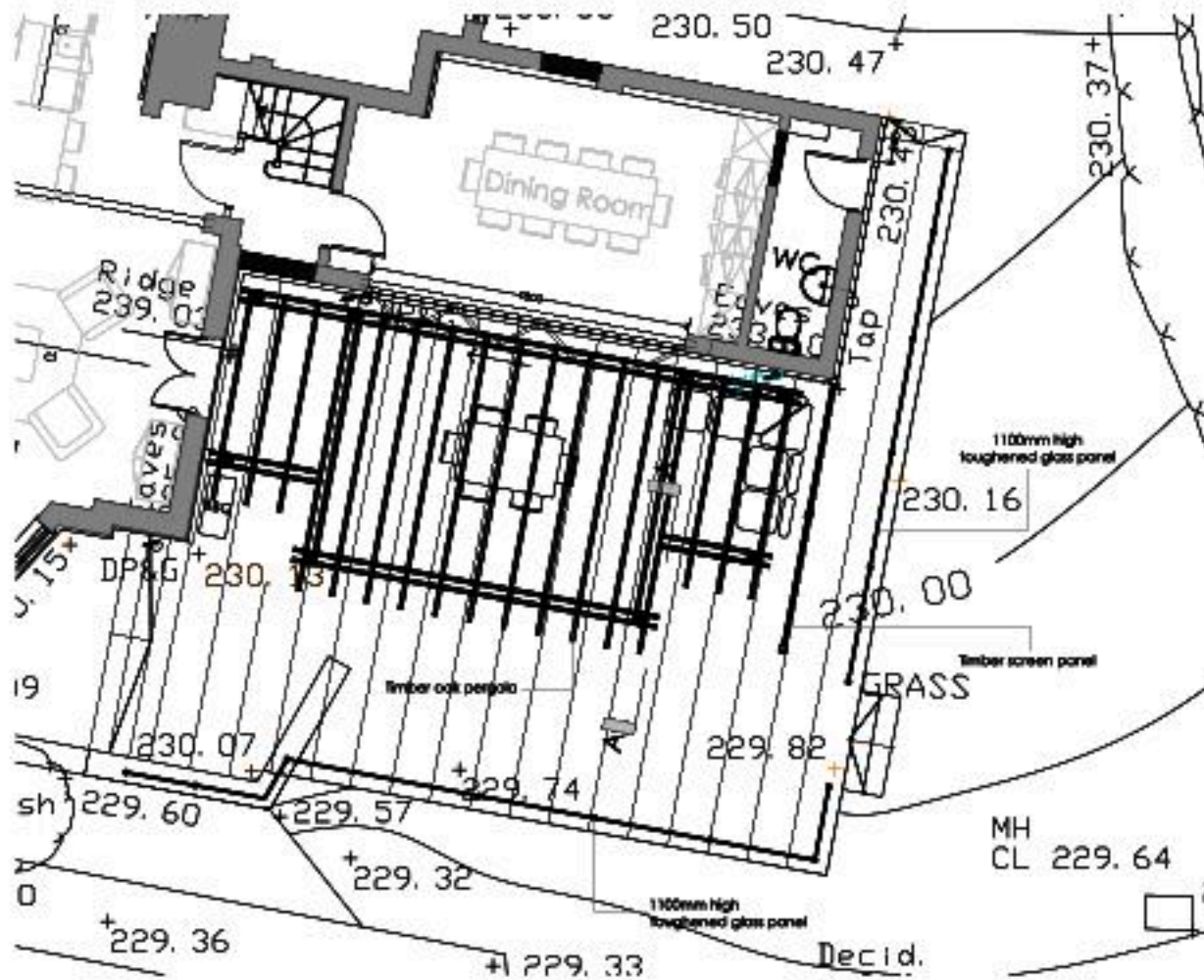
Proposed Plan Scale: 1:50
