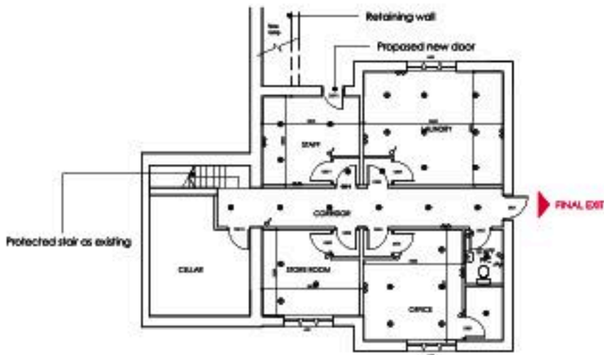
Proposed Basement Floor Plan
