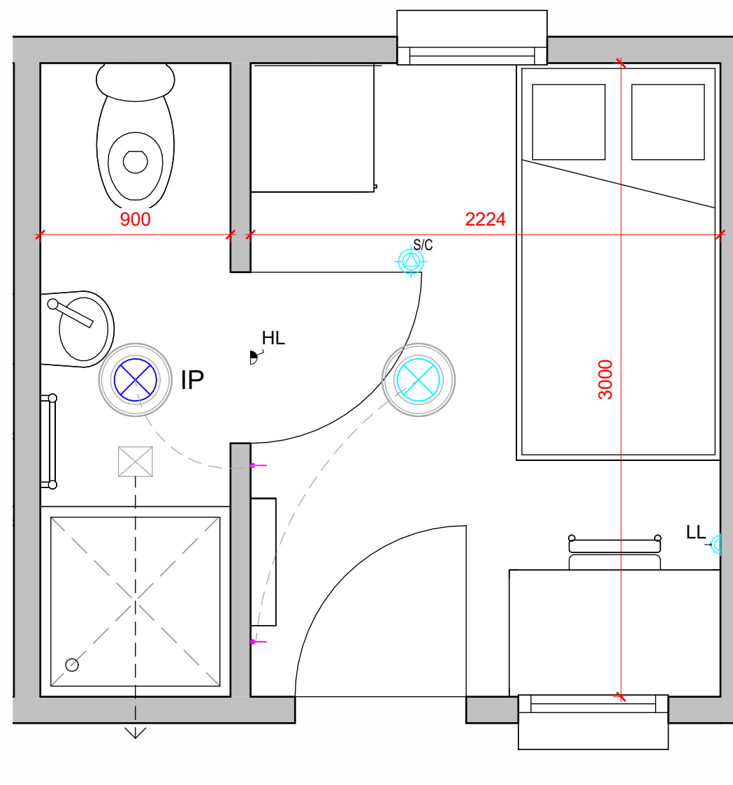
TYPICAL BEDROOM LAYOUT 1 : 25
