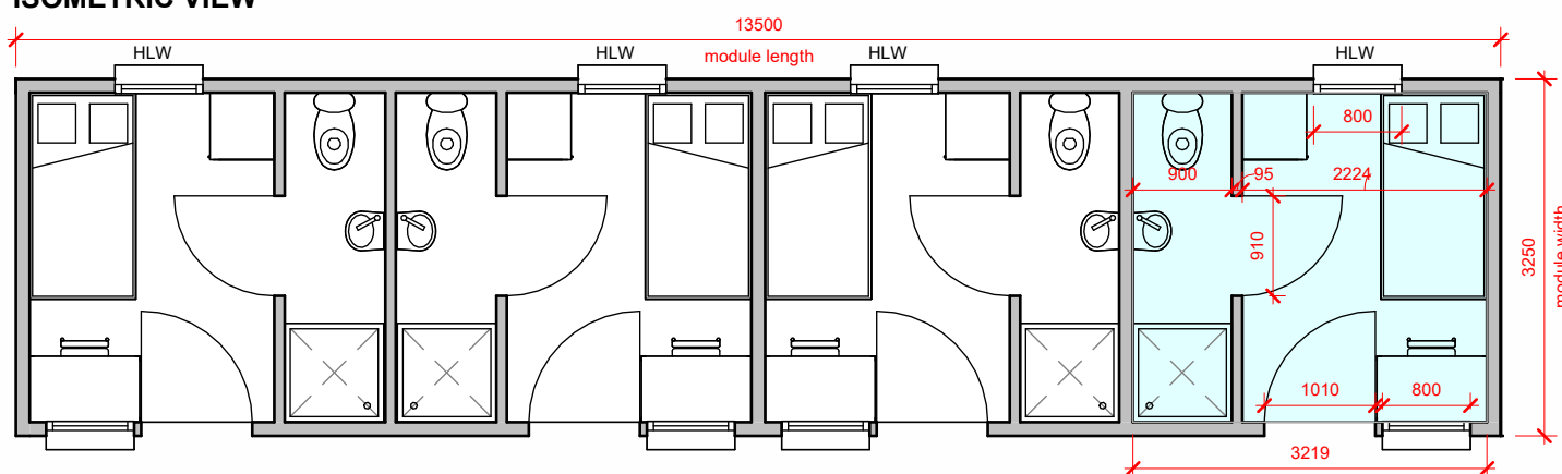
TYPICAL ROOM LAYOUT
