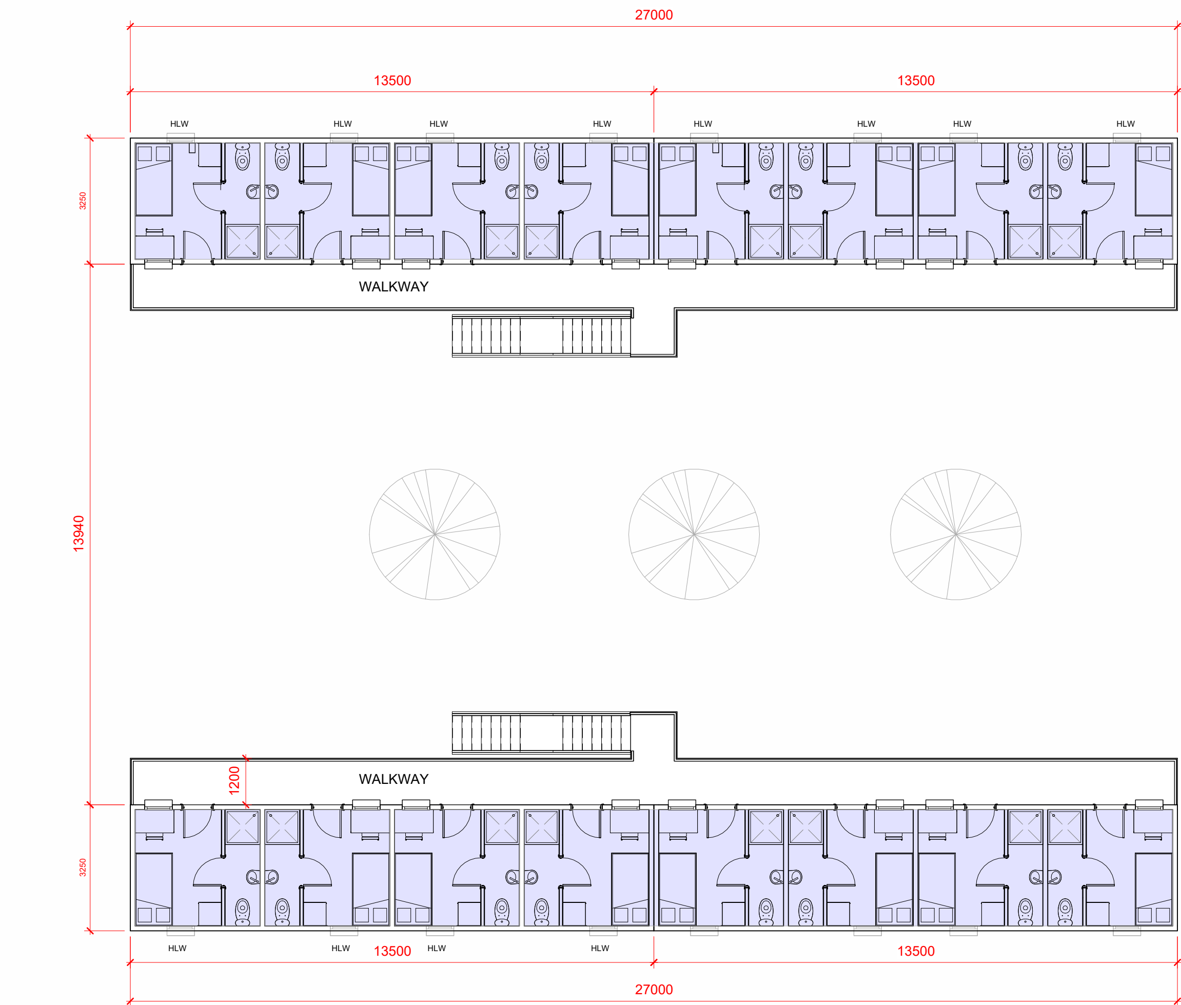
FIRST FLOOR PLAN 1 : 100
