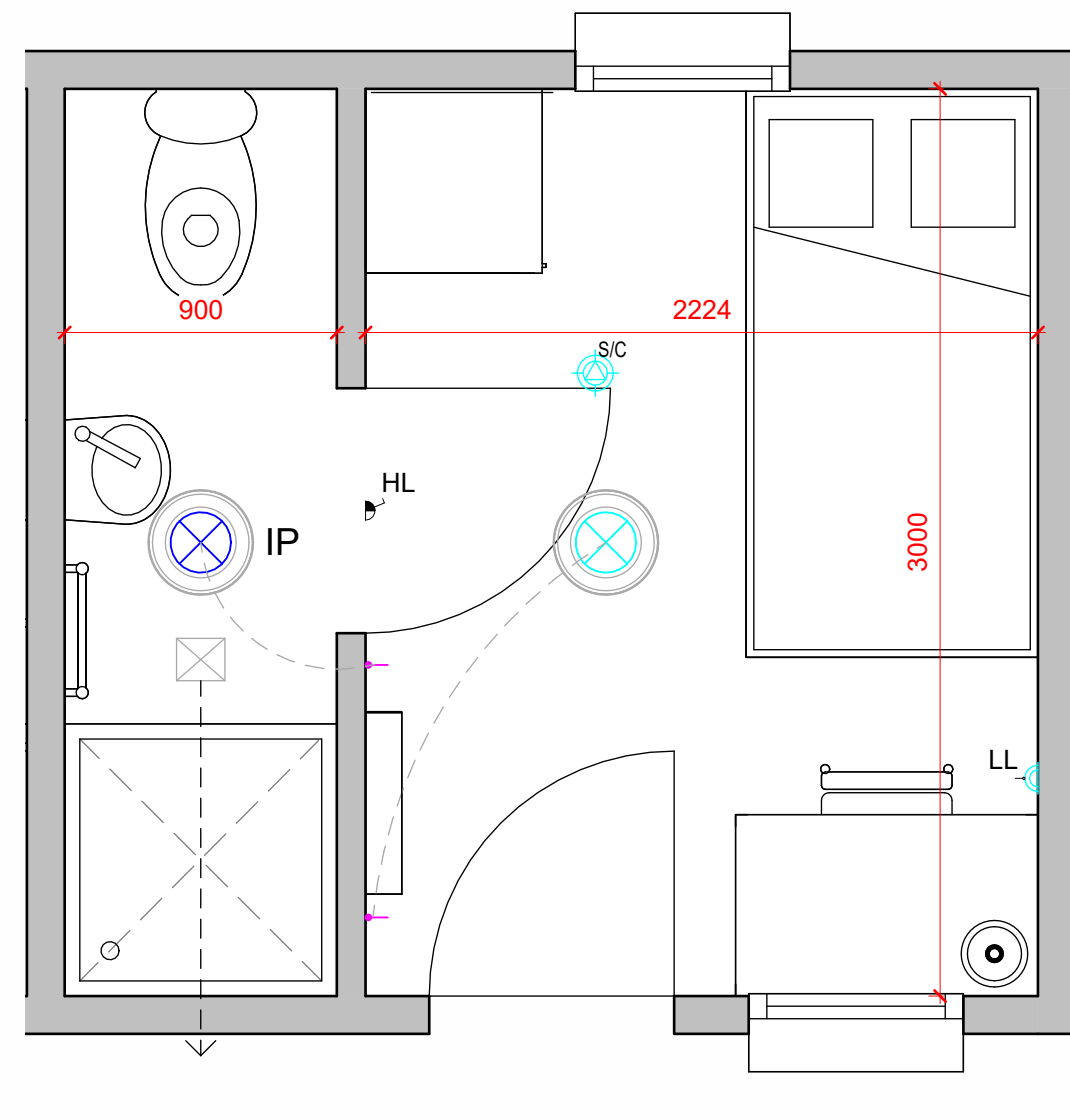
TYPICAL BEDROOM LAYOUT 1 : 25
