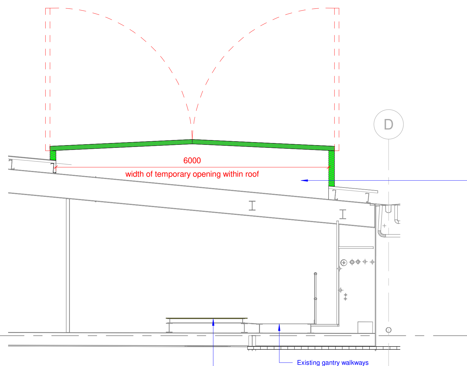
ROOF OPENING SECTION
