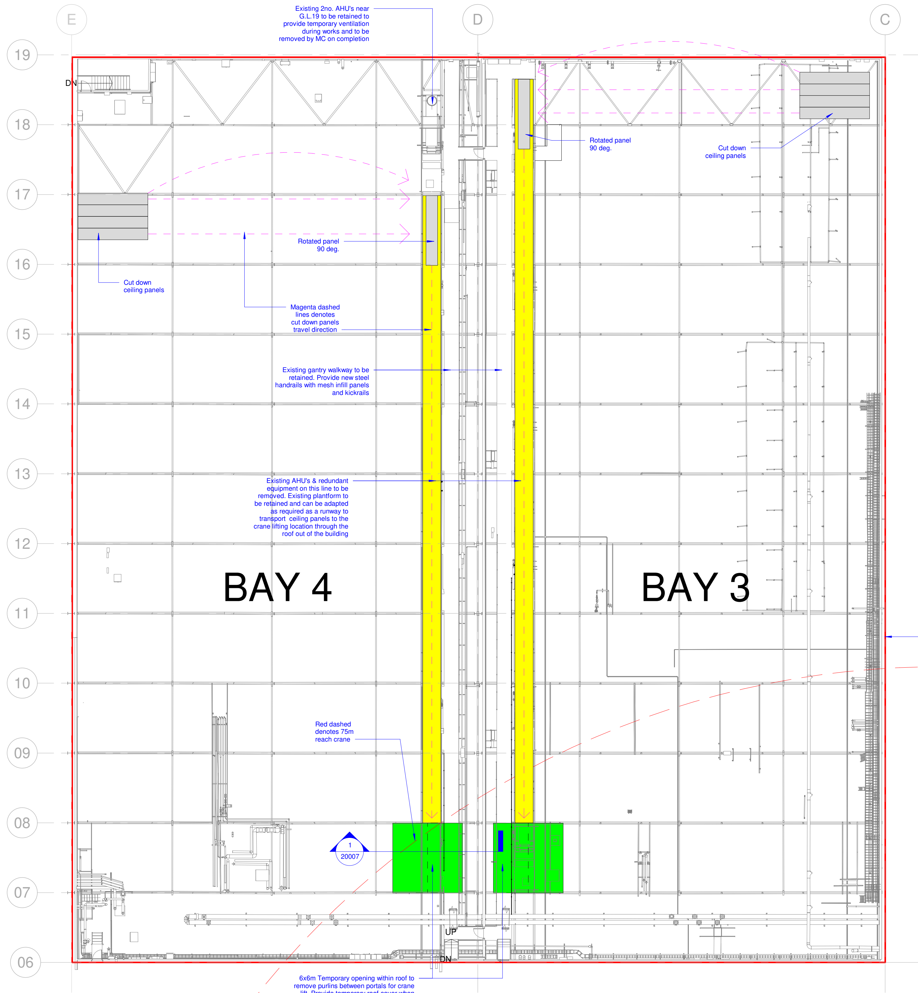
BAY 3 & 4 PROPOSED CEILING REMOVAL PLAN
