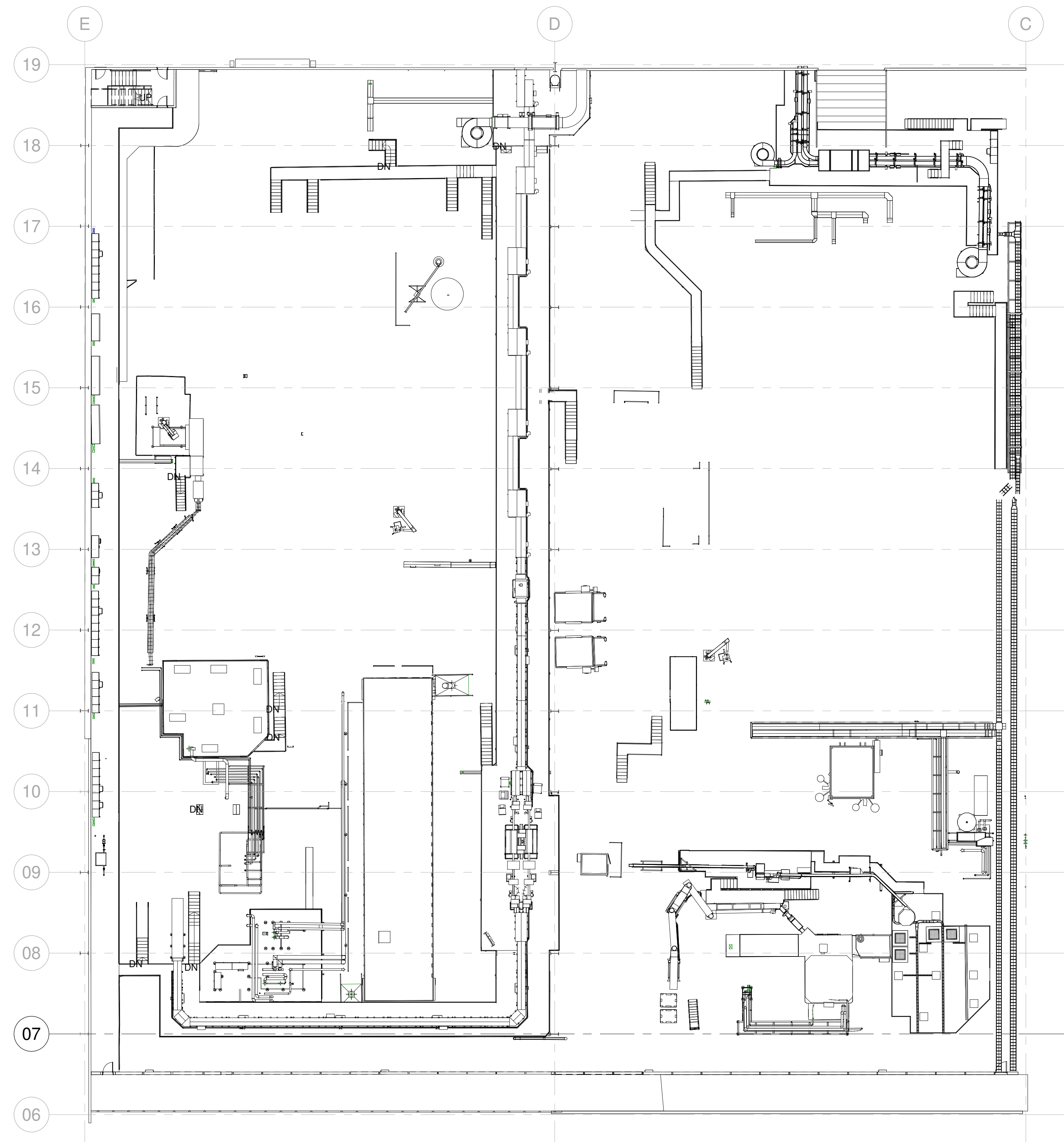
BAY 3 & 4 EXISTING GROUND FLOOR WALKWAYS
