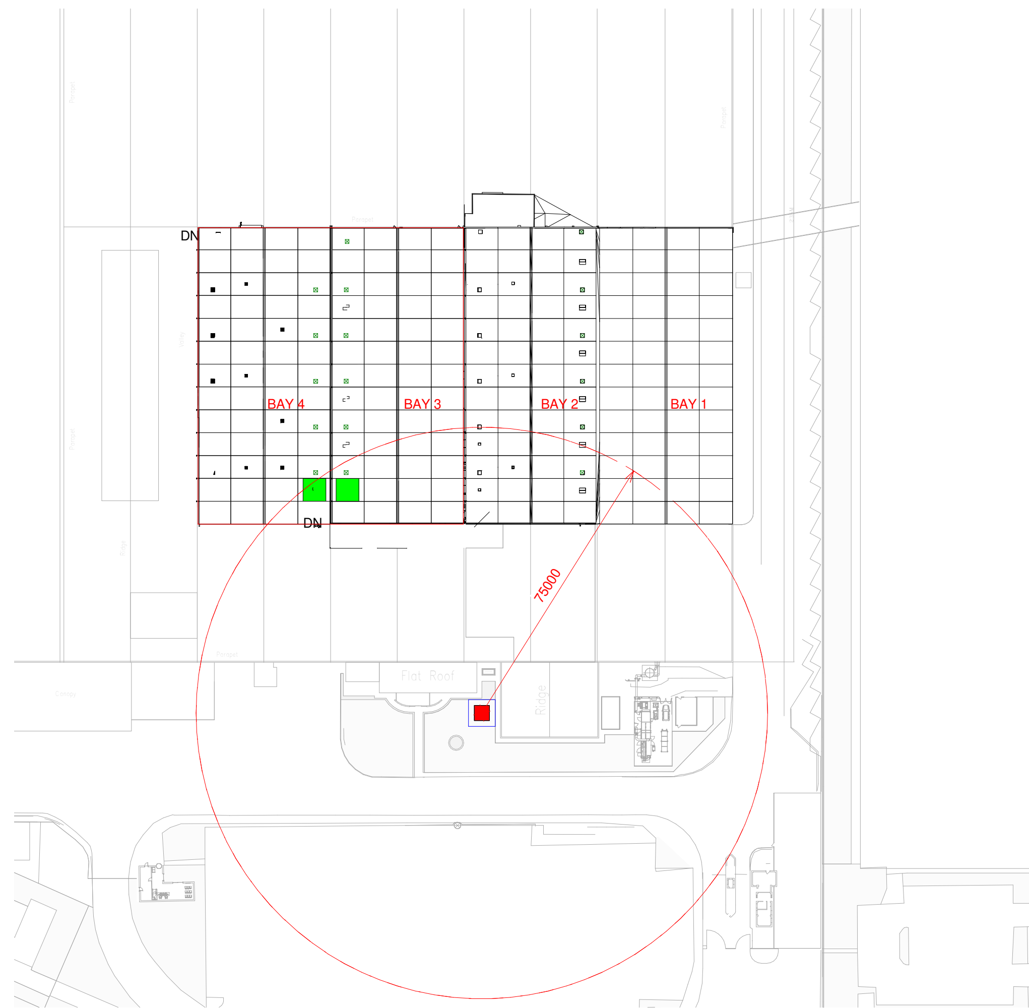
GA BUILDING ROOF PLAN
