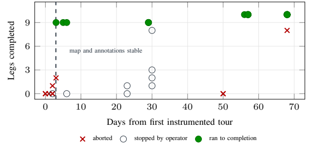
Fig. 6. All 47 instrumented guided tours over ten weeks. To the left of the rule, while the map and its annotations were still being edited, one navigation leg in seven succeeded and no tour finished. To the right, 308 of 309 legs succeeded and 29 tours ran end to end. Operator stops are not failures: every leg they had attempted had succeeded. The single late failure is an H4 event, described in Section VI-B.
