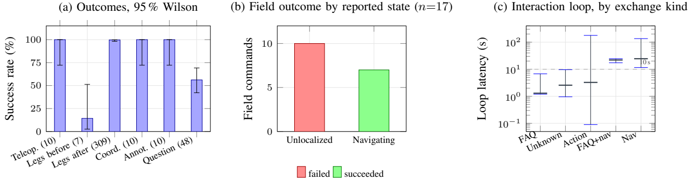
Fig. 5. (a) Every success rate reported in this paper, with its interval. The two leftmost tour bars contrast guided-tour legs before and after the map and its annotations stopped changing, the largest effect we measured; the coordinate and annotation arms of the bench comparison are indistinguishable ( p = 1.00 ). (b) In the field record, the state the robot reports separates success from failure perfectly, while the addressing scheme does not separate them at all. (c) Median and range of the interaction loop per exchange kind, log scale. Exchanges that only look up an answer sit below 10 s; those that also move the robot sit above it, because the preparation sequence runs inside the loop. A single pooled latency would describe neither group.
