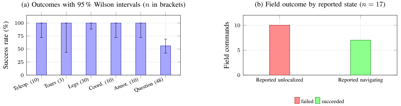
Fig. 6. (a) Measured outcomes. Intervals remain wide because samples are small. The two arms of the bench comparison are indistinguishable: identical success rates ( p = 1.00 ) and overlapping completion times ( p = 0.76 ). (b) In the field record, reported localization state separates success from failure perfectly, and the addressing scheme does not separate them at all.
