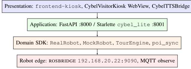
Fig. 3. Logical architecture (edge-first, no vendor cloud).
