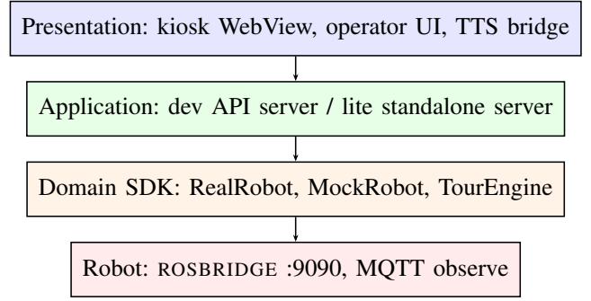
Fig. 3. Logical architecture (edge-first, no vendor cloud).
