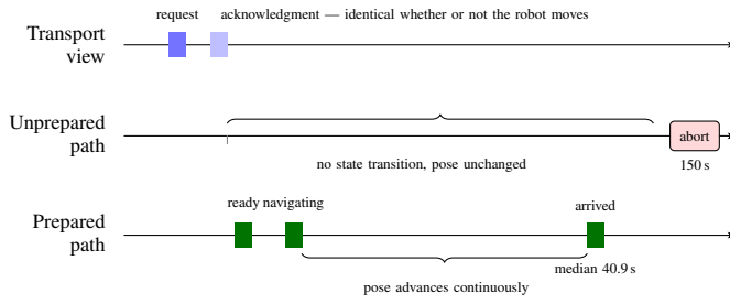
Fig. 4. The transport lane is identical whether or not the command executes. Only an independent state topic distinguishes the two lower cases. Timings from the bench comparison of Section VI-C ( n = 3 per arm).
