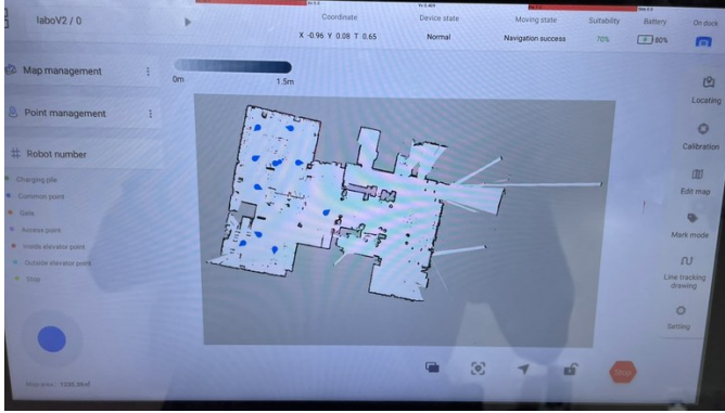
Fig. 5. The vendor deployment application showing the 1235 m 2 laboratory map used throughout this study, with its annotated points of interest. These annotations live in the chassis marker manager; reusing them avoids the drift that affects coordinates extracted offline, but does not by itself make navigation succeed (Section VI-C).
