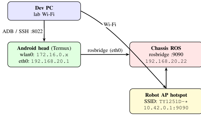
Fig. 2. Network topology on CIOT TY1251D-03195. CYBEL on Termux reaches ROSBRIDGE at 192.168.20.22 (internal eth0, preferred path). A dev PC can also reach the chassis directly via the robot's hotspot (10.42.0.1:9090). The head's DHCP address (172.16.0.x) must not be confused with the chassis IP.
