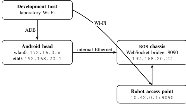
Fig. 2. Three network segments on a product marketed as a single device. Conflating the head's DHCP address with the chassis address was the most frequent operator error we observed.
