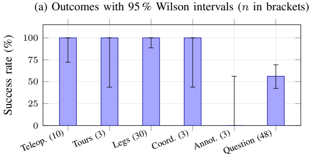
Fig. 6. (a) Measured outcomes. Intervals are wide because samples are small; the annotation arm of the bench comparison and the coordinate arm do not separate at p = 0.10 . (b) In the field record, reported localization state separates success from failure perfectly, and the addressing scheme does not separate them at all.
