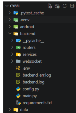
FIGURE 21 – architecture Backend
