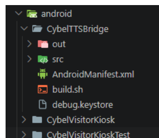
FIGURE 23 – Architecture Android
