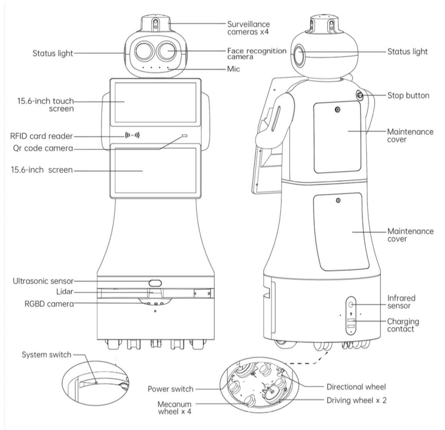
FIGURE 20 – Structure du robot
