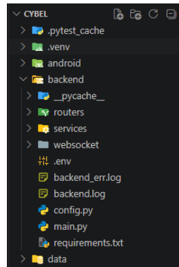
FIGURE 21 – architecture Backend
