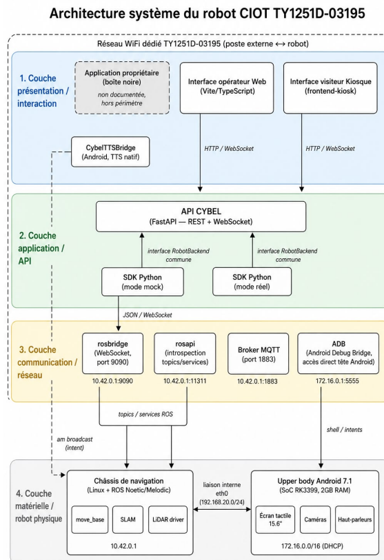
FIGURE 3 – Architecture système globale du robot CIOT TY1251D-03195
