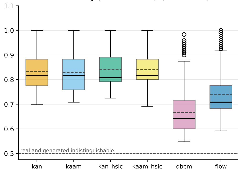
RF accuracy (interventional) (0.5 is ideal)
