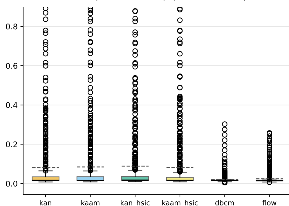
MMD (interventional) (lower is better)
