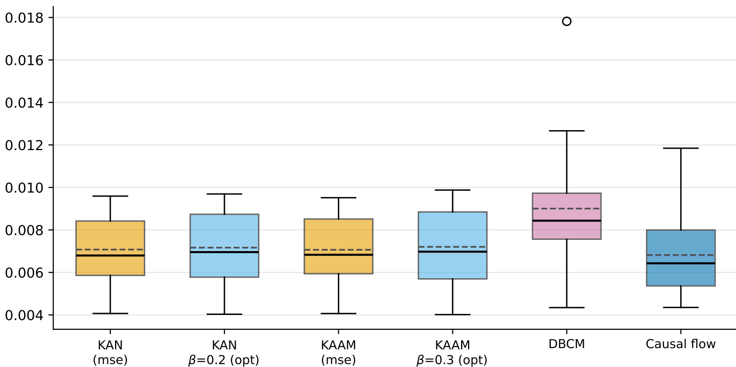
MMD (observational) (lower is better)
