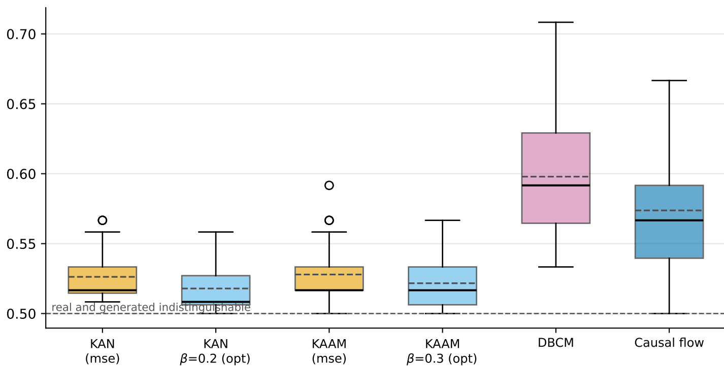
RF accuracy (observational) (0.5 is ideal)
