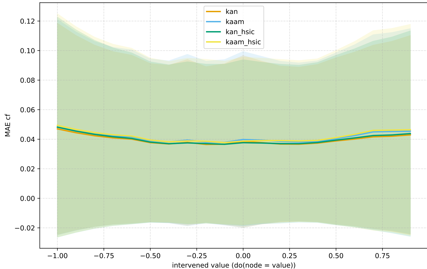
MAE cf vs intervention value (over 11 nodes)
