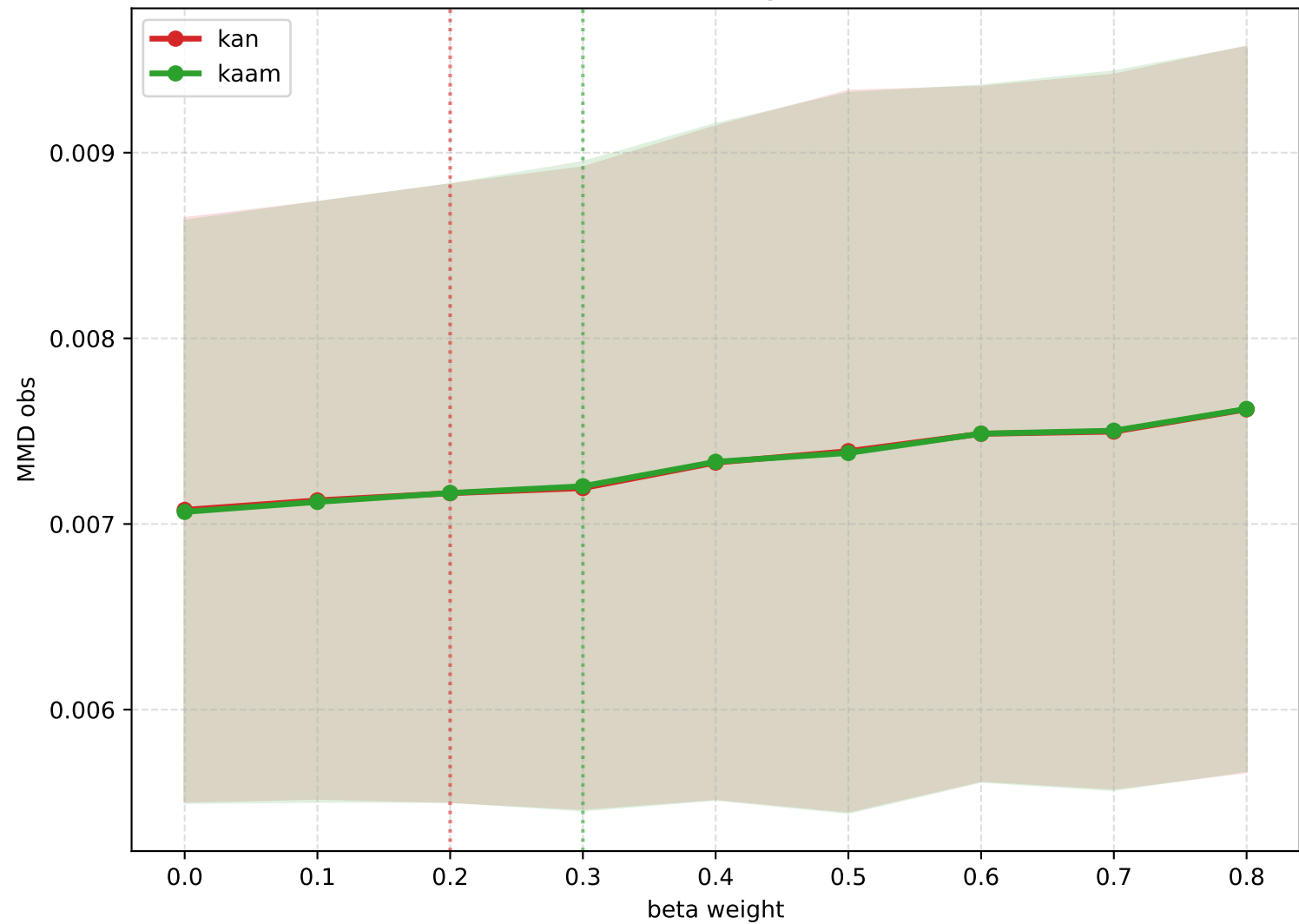
MMD obs vs beta weight (20 seeds)
