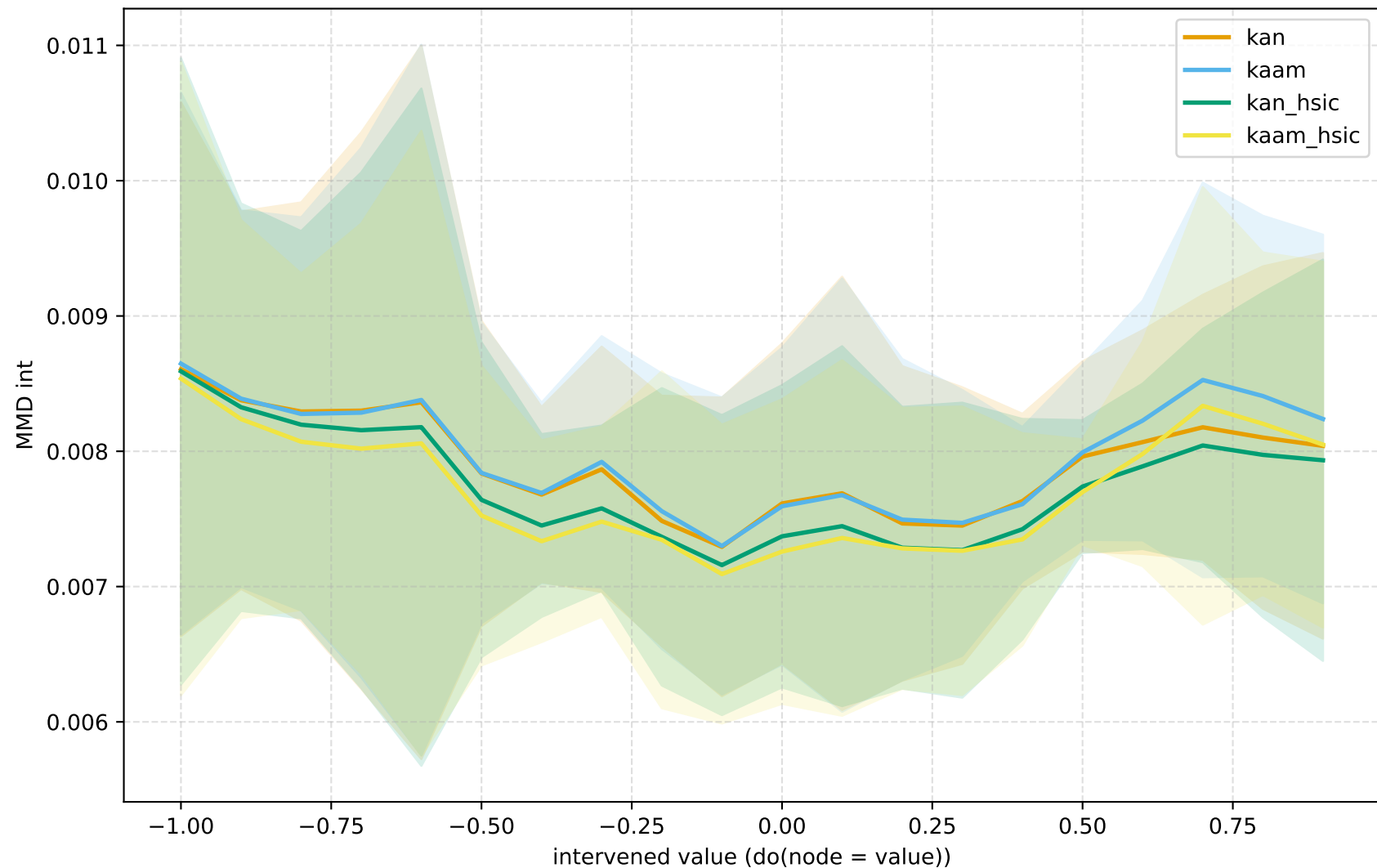
MMD int vs intervention value (over 11 nodes)
