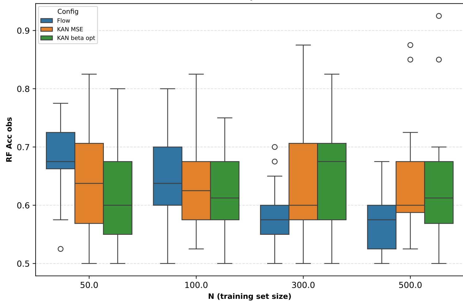
RF Acc obs boxplot (20 seeds)
