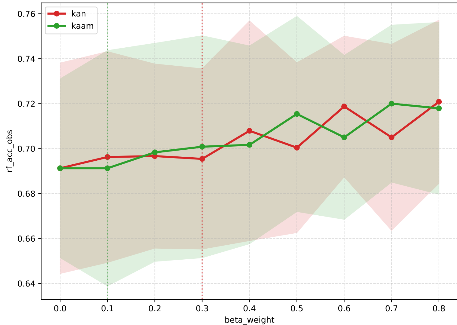
RF accuracy with respect to beta weight (media \pm std, 20 semillas)
