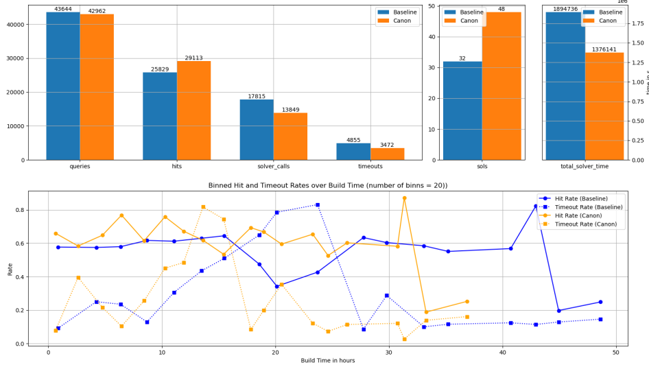
Figure 3: Compares cache metrics collected during the compilation of libgmp using the unmodified Minotaur (baseline in blue) and the extended Minotaur (canon in orange). The top row shows the total number of queries (queries), cache hits (hits), solver calls after cache misses (solver_calls), solver timeouts (timeouts), rewrites successfully queried from the cache (sols), and time spent in the solver (total_solver_time) across all build units.
