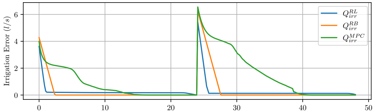
RL-based WF-MS
