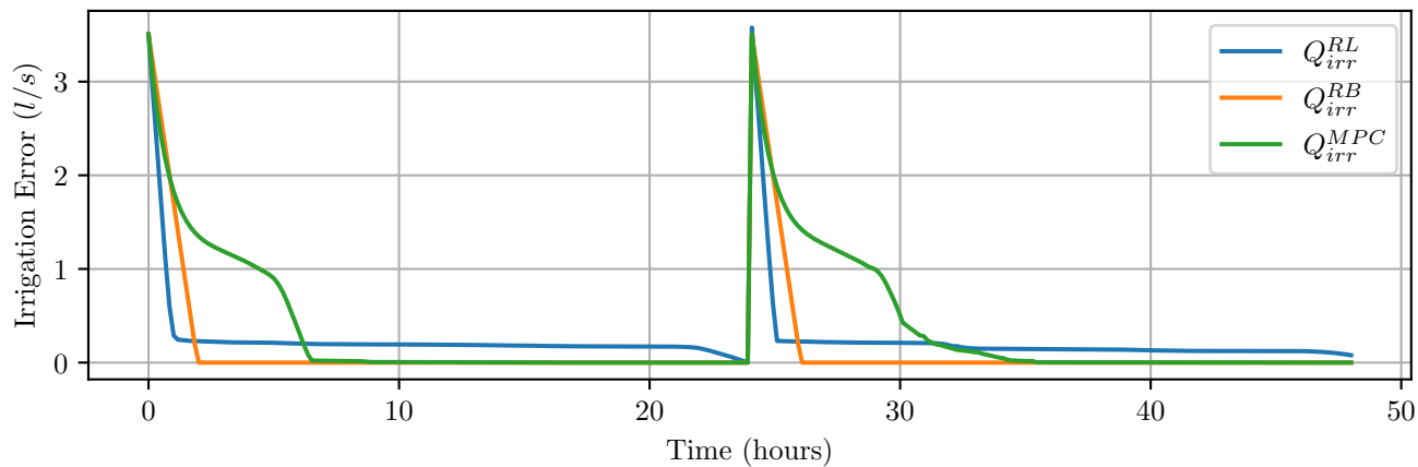
RL-based WF-MS
