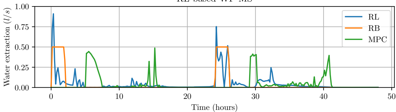
RL-based WF-MS
