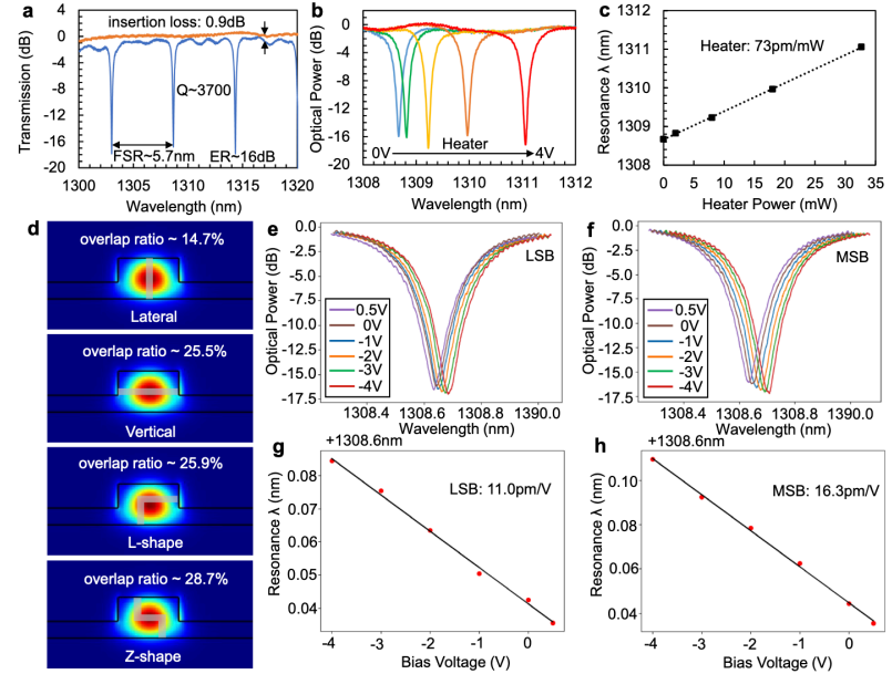
Fig. 2 | Direct current (DC) characteristics of a single microring modulator (MRM). a , Measured transmission spectrum of a single-channel MRM (blue) and a pair of grating couplers (orange). b , Measured transmission spectrum versus heater voltage ranging from 0 V to 4 V. c , Resonance wavelength versus heater power. d , Calculated overlap ratios between the waveguide transverse electric (TE) mode and depletion regions of different junctions. e , f , Measured transmission spectrum versus junction voltage from 0.5 V to 4 V at the least significant bit (LSB) and most significant bit (MSB). g , h , Extracted resonance wavelengths versus junction voltage for LSB and MSB.
