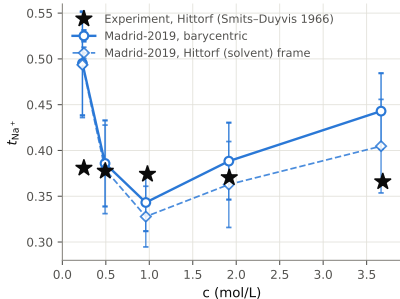
b Cation transport number
