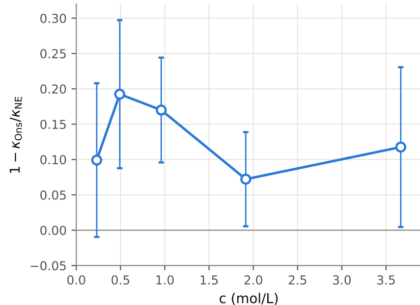
a Ion-correlation reduction of \kappa
