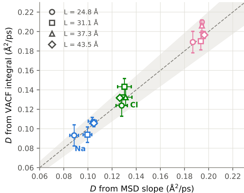
b Einstein vs Green-Kubo (11/12 within 2\sigma )
