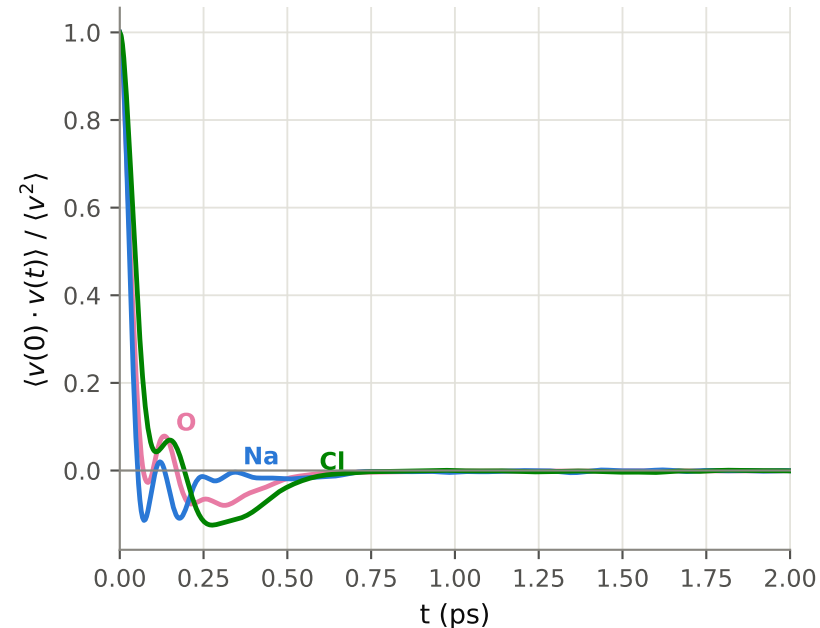
a Velocity autocorrelation ( L = 43.5 \text{ \AA} , seed avg.)
