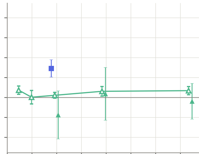
Cl-Cl distinct
