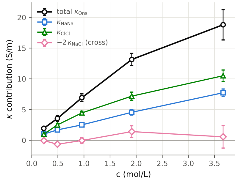
a Onsager decomposition of \kappa ( z = \pm 1 )
