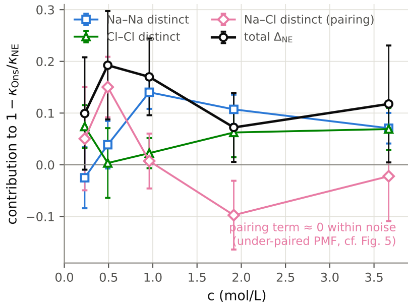
b Origin of the Nernst-Einstein deviation
