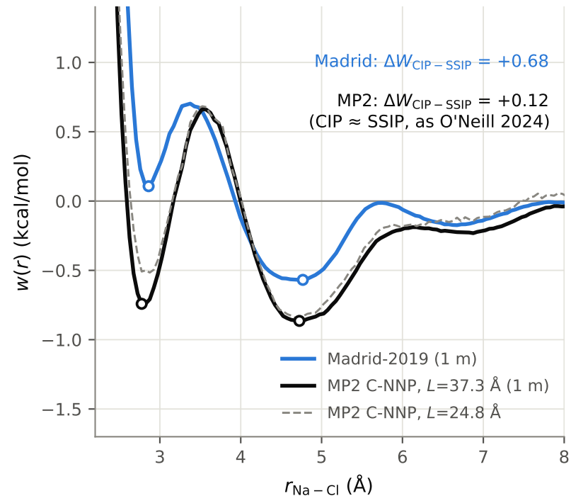
Na-Cl pairing free energy, 1 m
