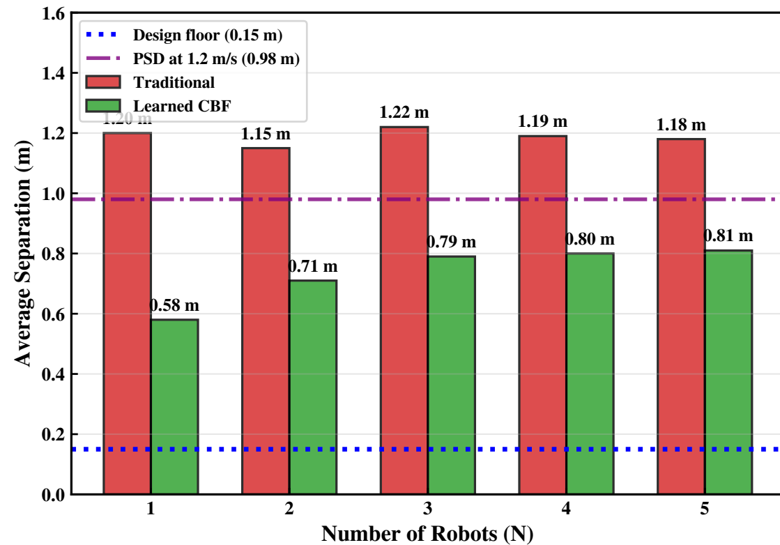
Human-Robot Separation Distance
