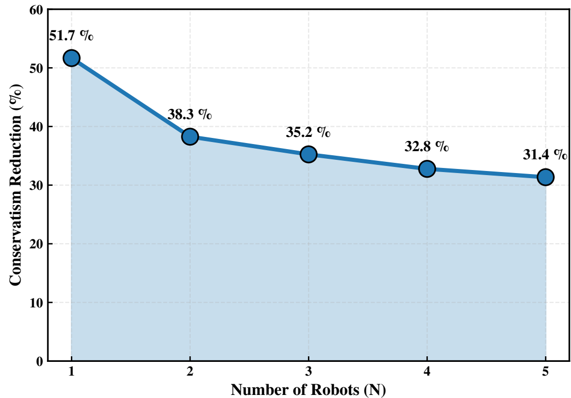
Reduction in Separation Conservatism (51.7 % at N = 1 to 31.4 % at N = 5)
