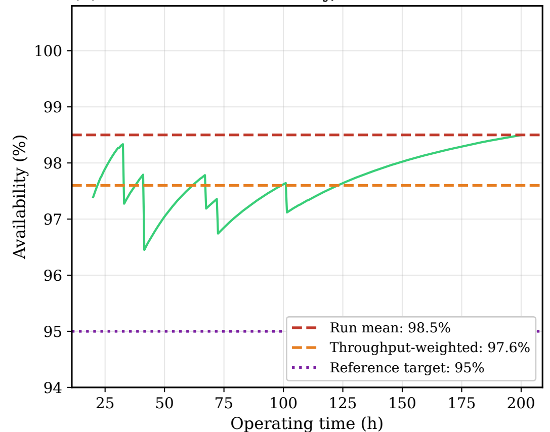
(b) Cumulative availability, 200 h simulated run
