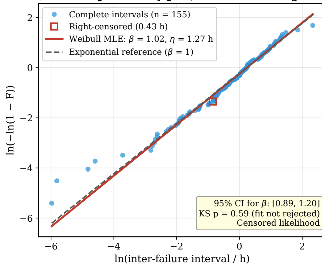
(a) Weibull probability plot, service-affecting faults
