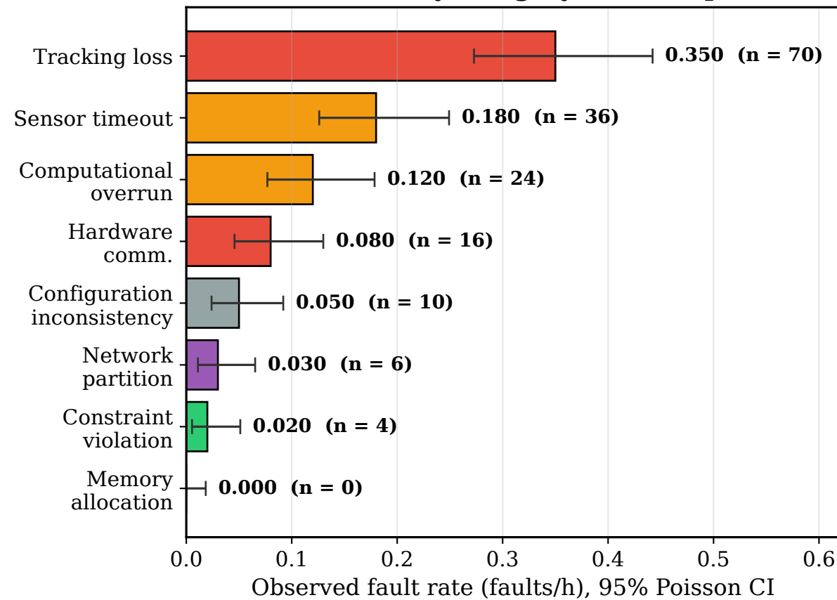
(c) Fault rate by category, 200 h exposure
