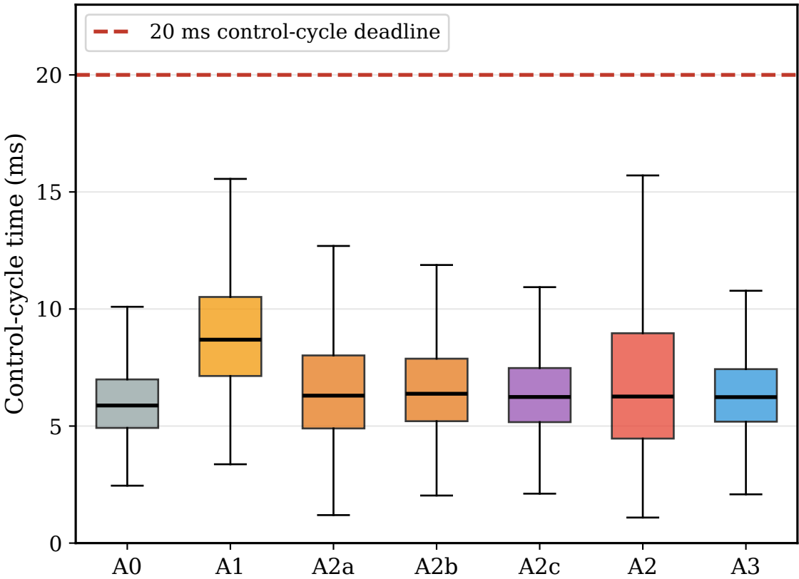
(a) Pooled cycle-time distribution, 30 condition cells per configuration
