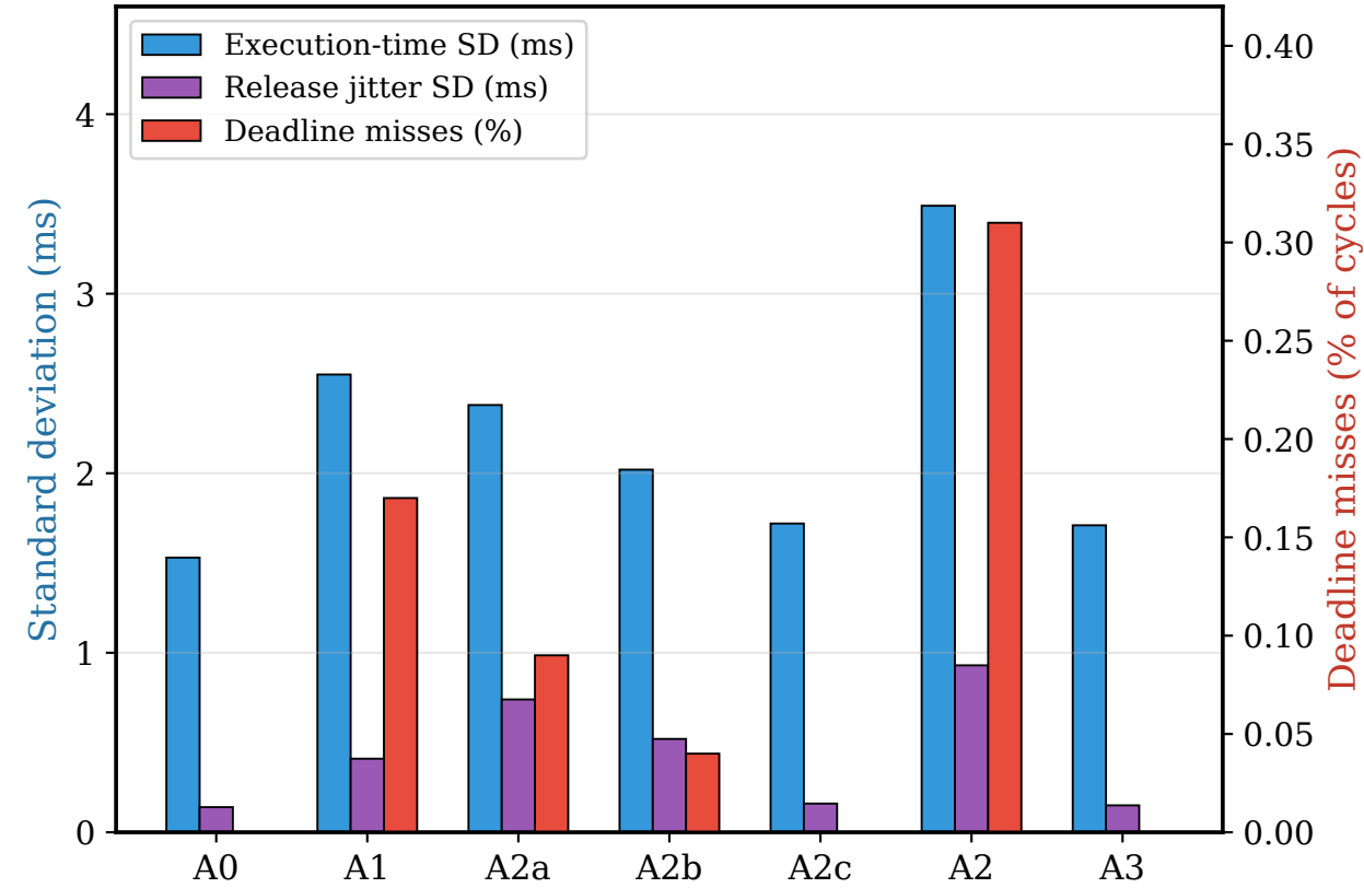
(c) Execution-time dispersion and release jitter are different quantities
