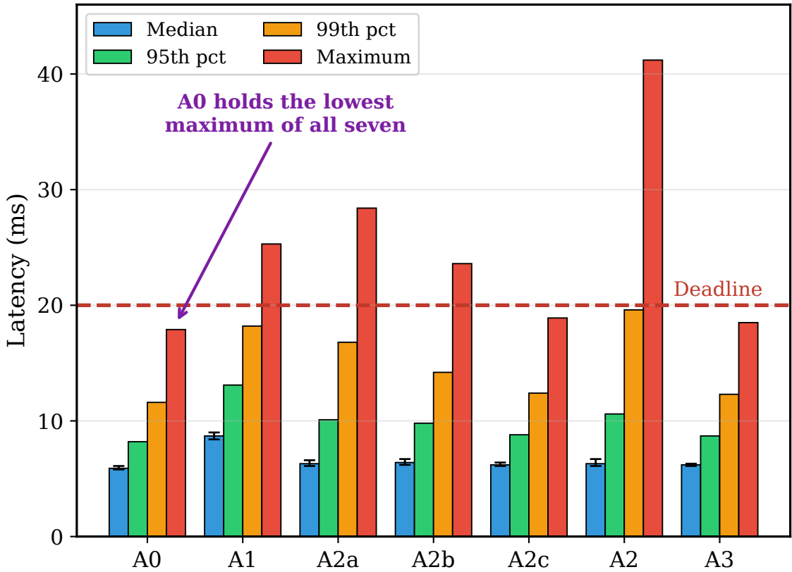
(b) Tail latency; bars on the median are bootstrap intervals over 30 runs
