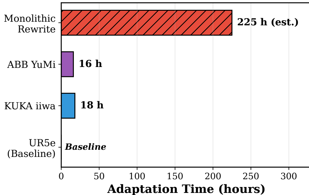
(b) Platform adaptation effort (measured vs. estimated)
