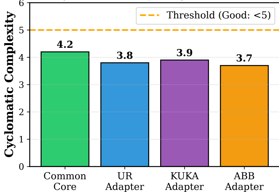
(c) Cyclomatic complexity (all below 5.0)
