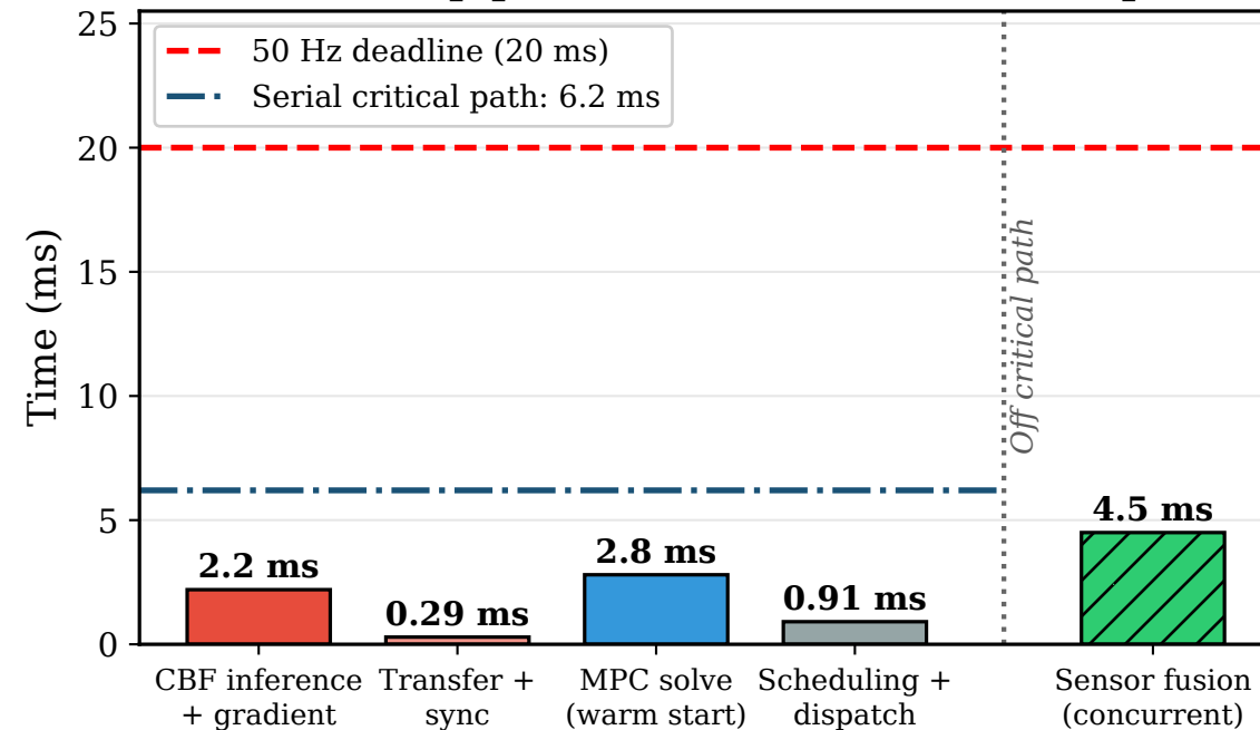
(b) Control pipeline: 6.2 ms serial critical path
