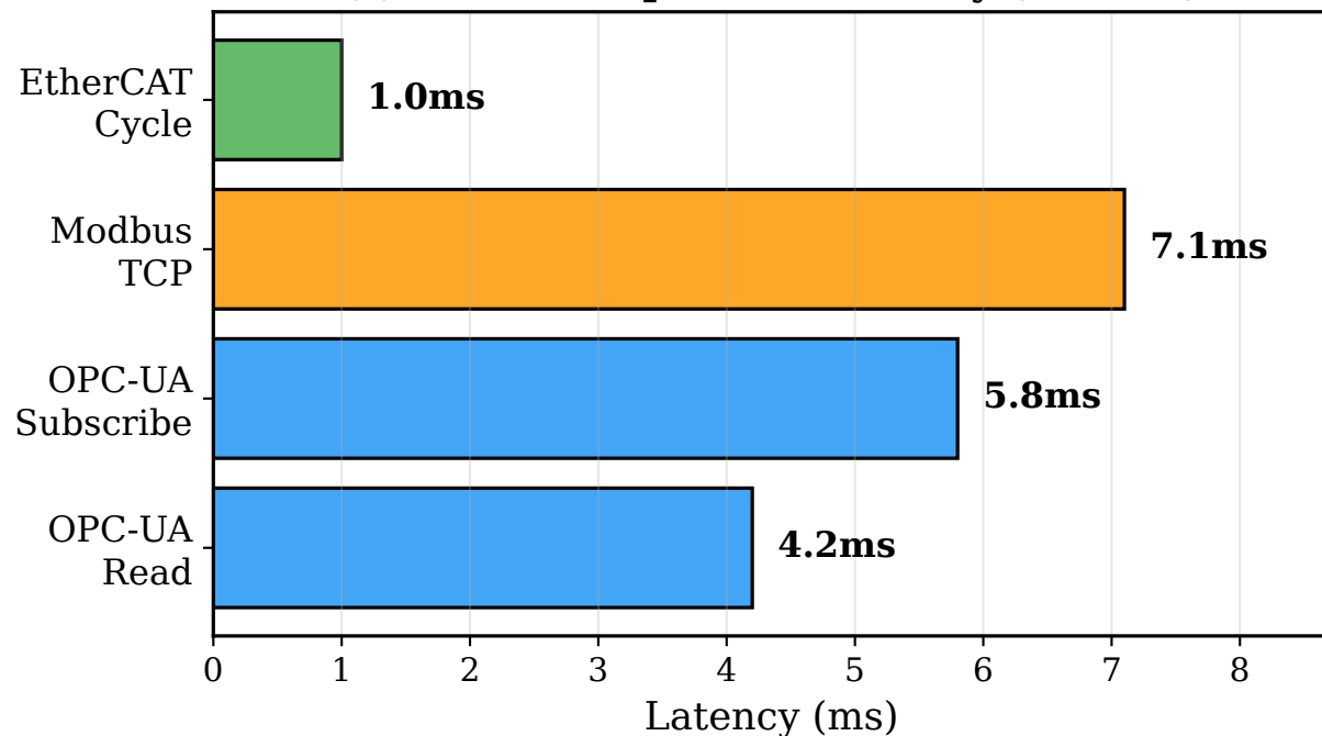
(c) Industrial protocol latency (median)
