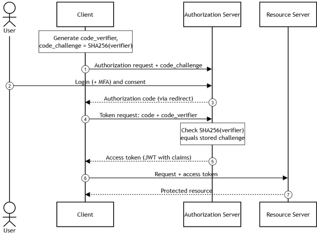
Figure 1: A typical IAM flow
