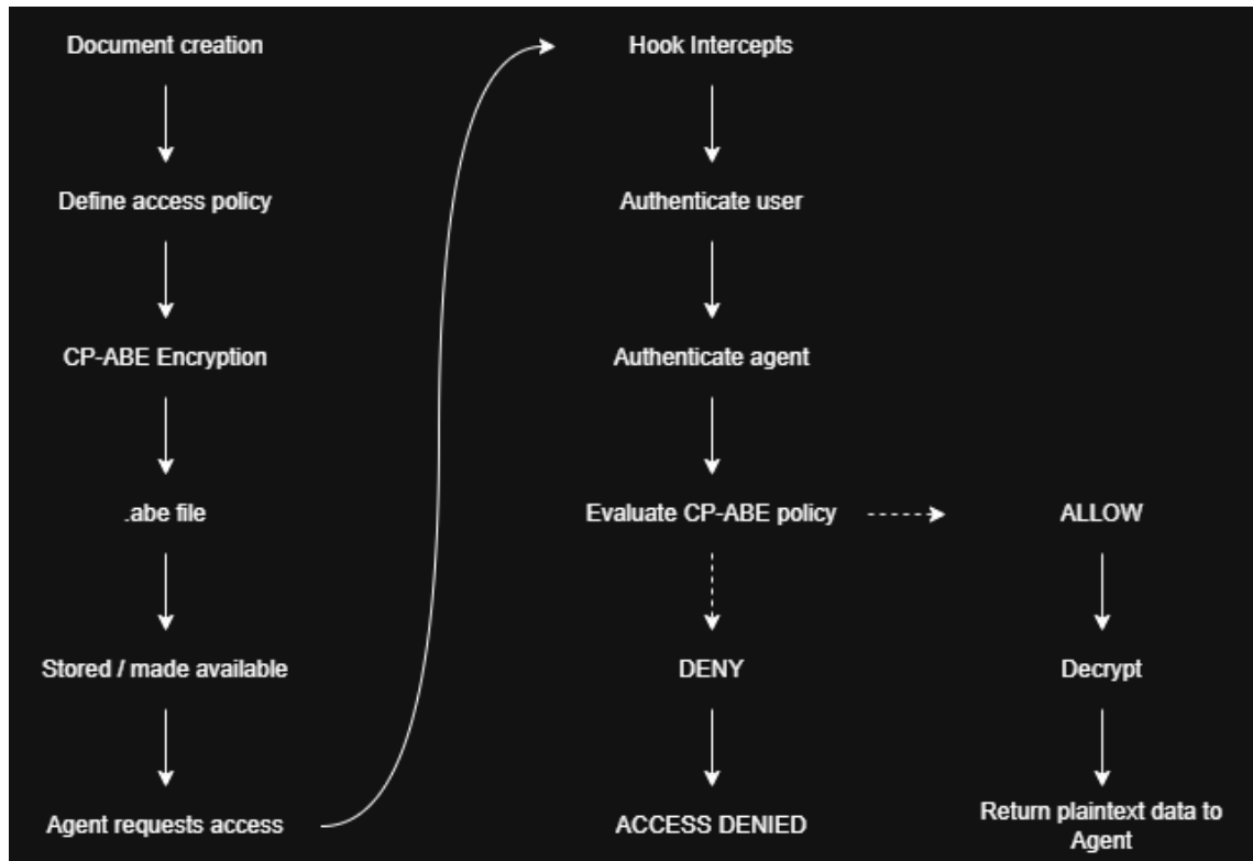
Figure 2: The flow diagram of the document lifecycle
