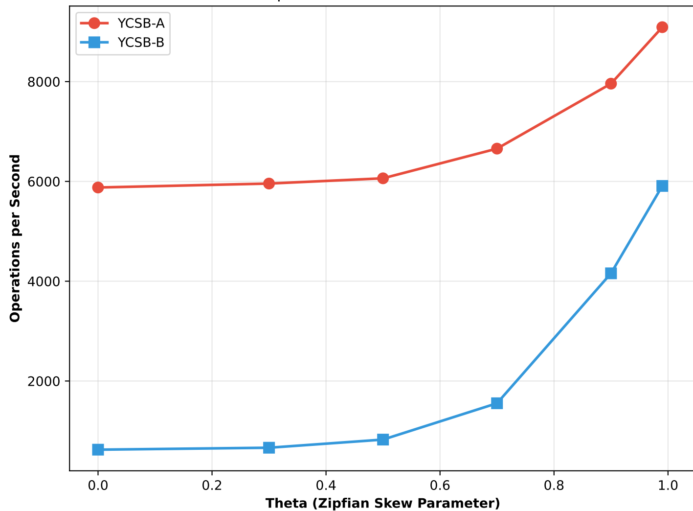
Total Operation Rate vs Contention Level
