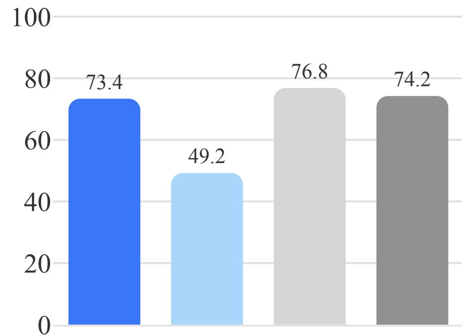
MMLU-Pro
