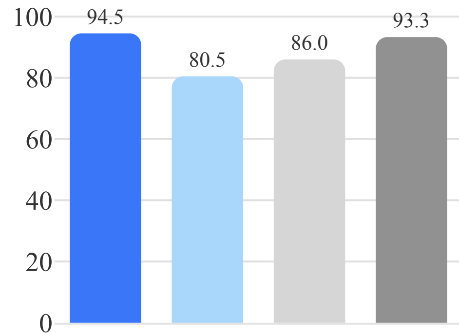
HumanEval
