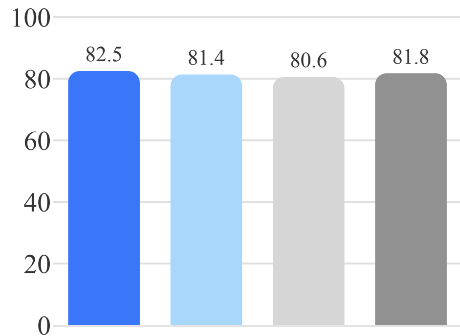
Spider
