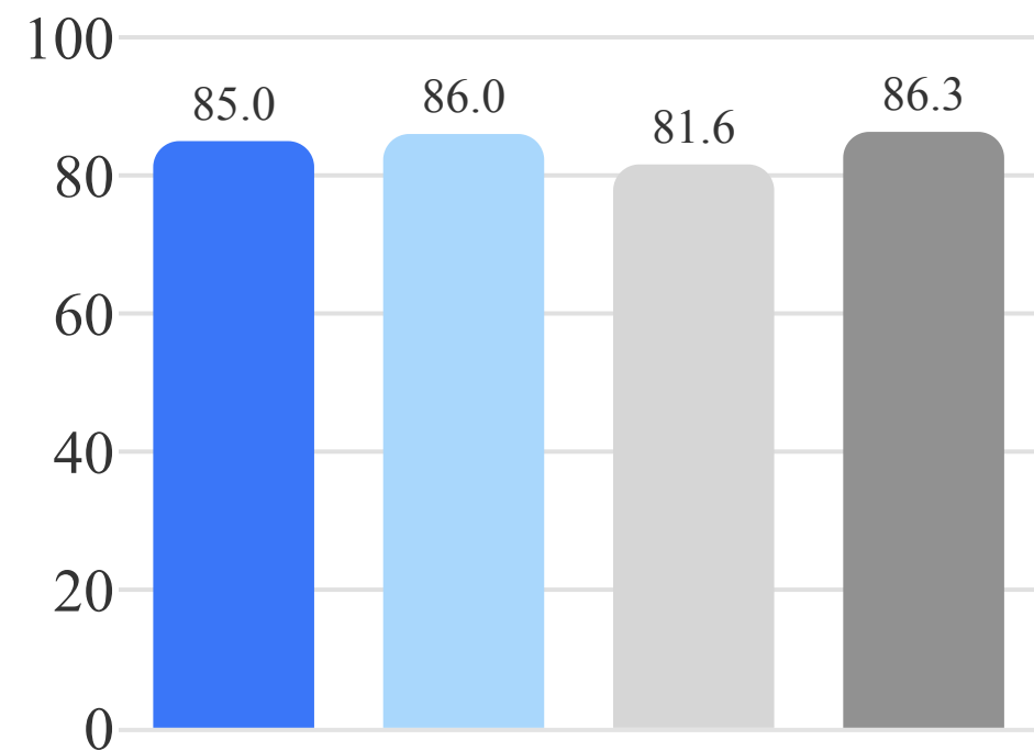
HellaSwag
