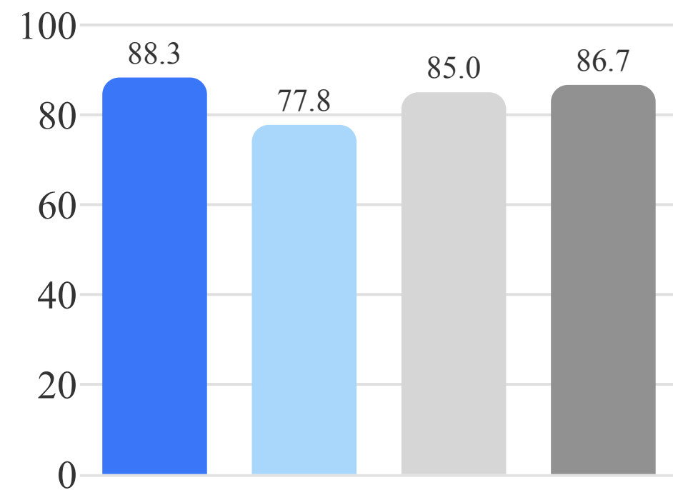
MBPP
