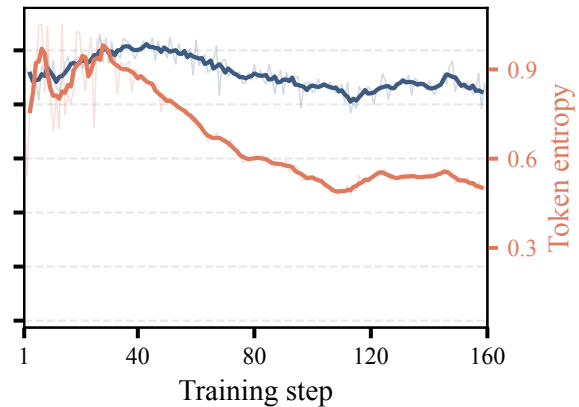
DCPO w/ CalibSFT
