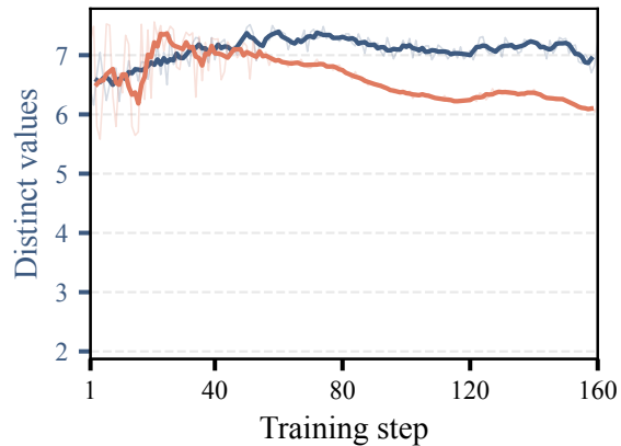
RLCR w/ CalibSFT
