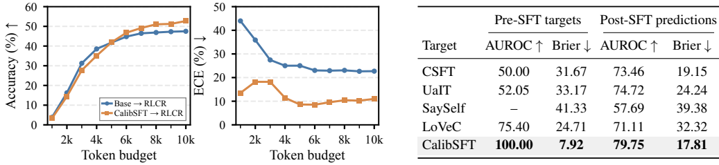
Figure 5: Accuracy (left) and ECE (right) on AIME’26 across token budgets for RLCR with and without CalibSFT initialization. CalibSFT yields substantially lower ECE across all budgets while matching accuracy at medium budgets and improving it at larger budgets.
