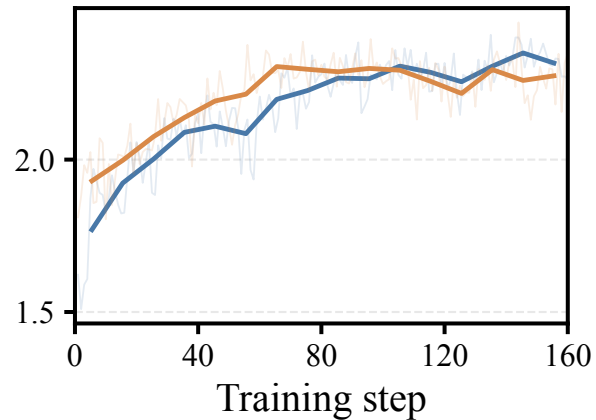
Total reward
