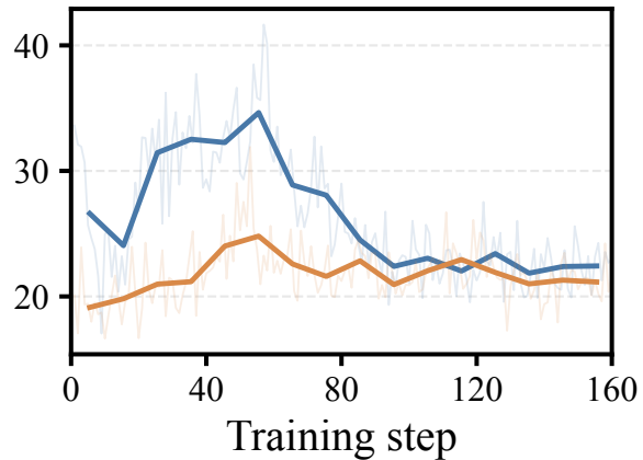
Brier score
