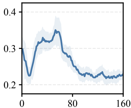
Brier loss ↓
