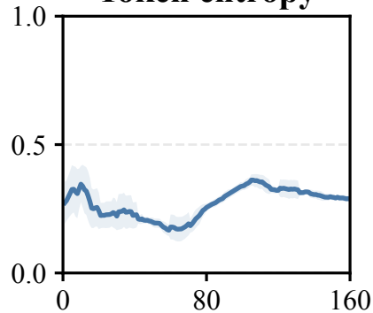
Token entropy
