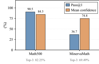
Figure 3: Performance comparison on Math500 and MinervaMath of RLCR on Qwen3-8B. Confidence differs little despite their large accuracy gap.
