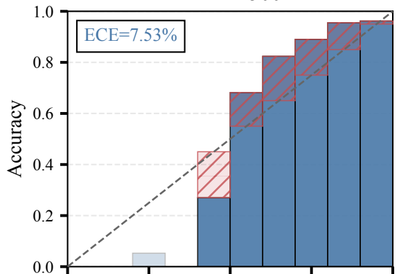
MATH-500
