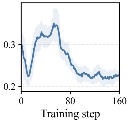
Brier loss ↓
