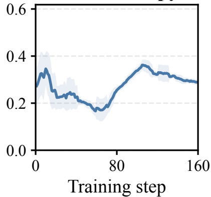
Token entropy
