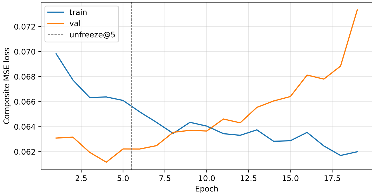
Training curves - caffeine
