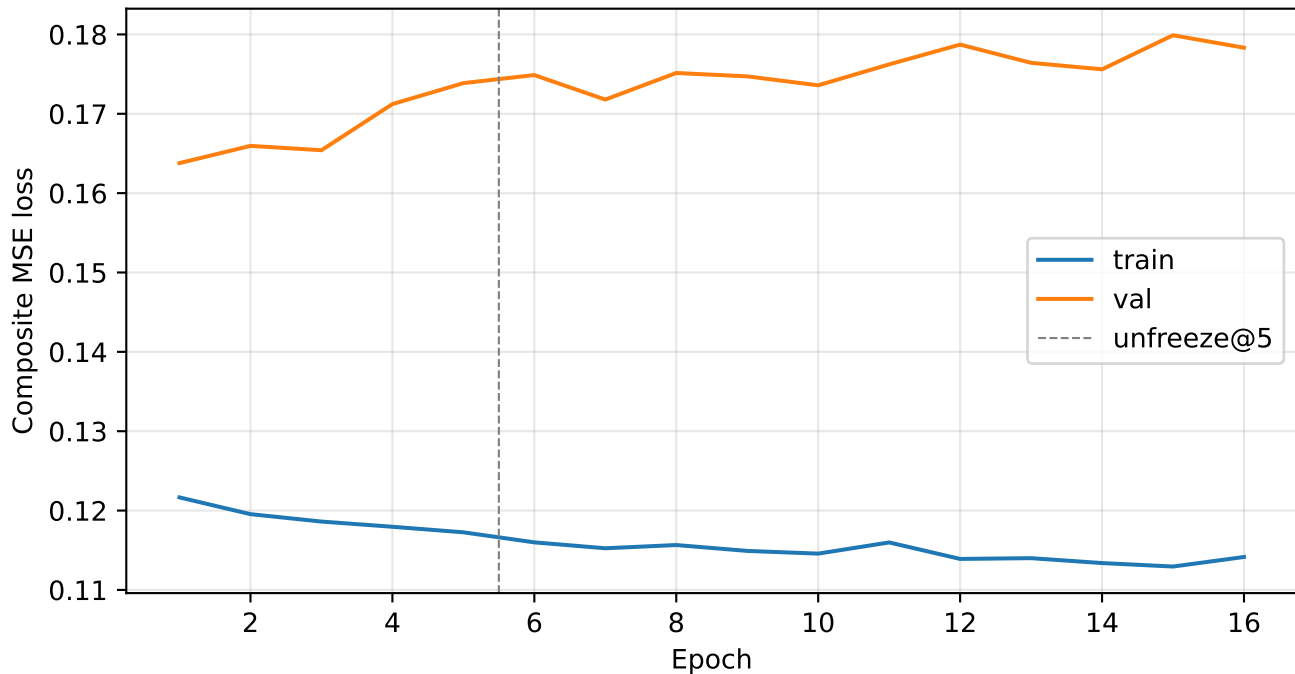
Training curves - digoxin
